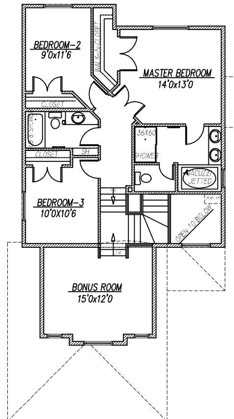
UPPER FLOOR PLAN 968 SQ.FT.
