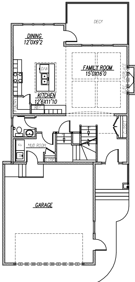
MAIN FLOOR PLAN 875 SQ.FT.
